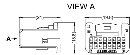
16 PIN FEMALE MATING FACE CONNECTOR - 1318386-1 PIN - 1123343-1
